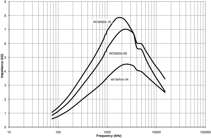
Common Mode Noise Impedance WCM-08,-09,-10
