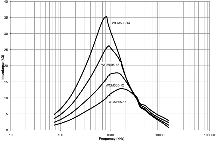
Common Mode Noise Impedance WCM-11,-12,-13,-14
