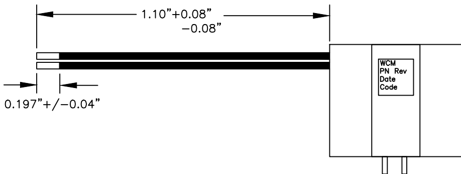
SIDE VIEW
