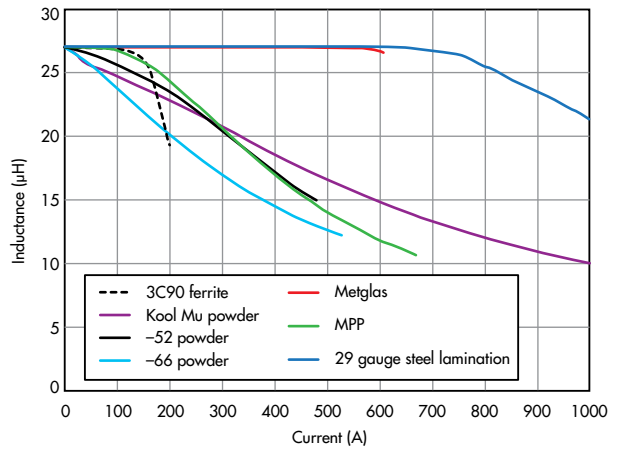
2. Based on simulation models, low-Bsat core materials exhibit a loss of inductance as Idc increases.
