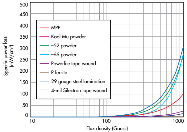
3. Taking frequency into consideration, each core material exhibits a different level of power loss at 10 kHz. The data from this chart comes from the core manufacturer's loss curves.
