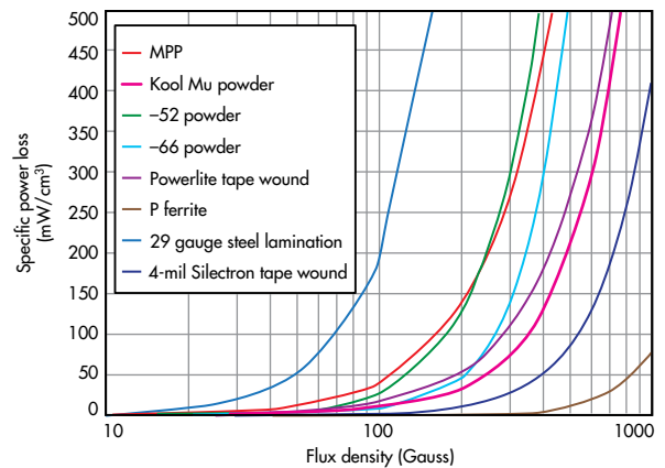
4. Core losses for various materials widen as frequency jumps to 100 kHz. The data from this chart comes from the core manufacturer's loss curves.
