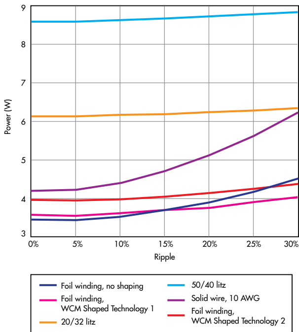
7. As a result of ac ripple currents at the fundamental frequency, power losses through the inductor winding increase with both frequency and ripple current. Compare the losses here at 10 kHz with those at 100 kHz in Figure 8.
